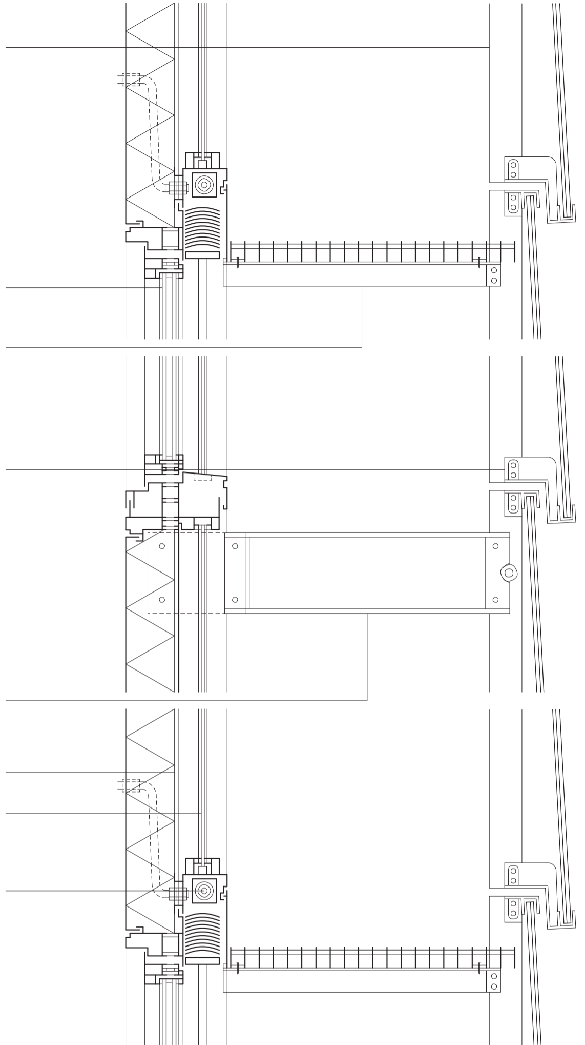
Vertical section - B wall
