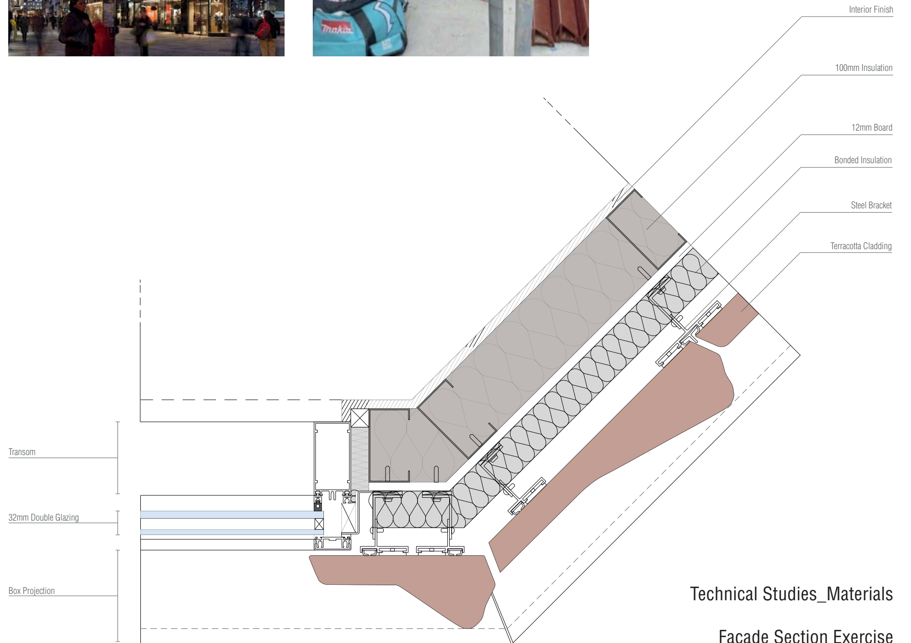
Facade Section (Plan)
